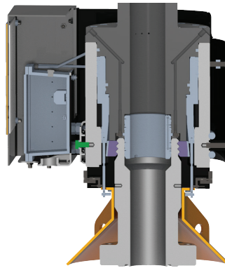
COMPACT SYSTEM WITH INTERNAL LOCK (RING)
