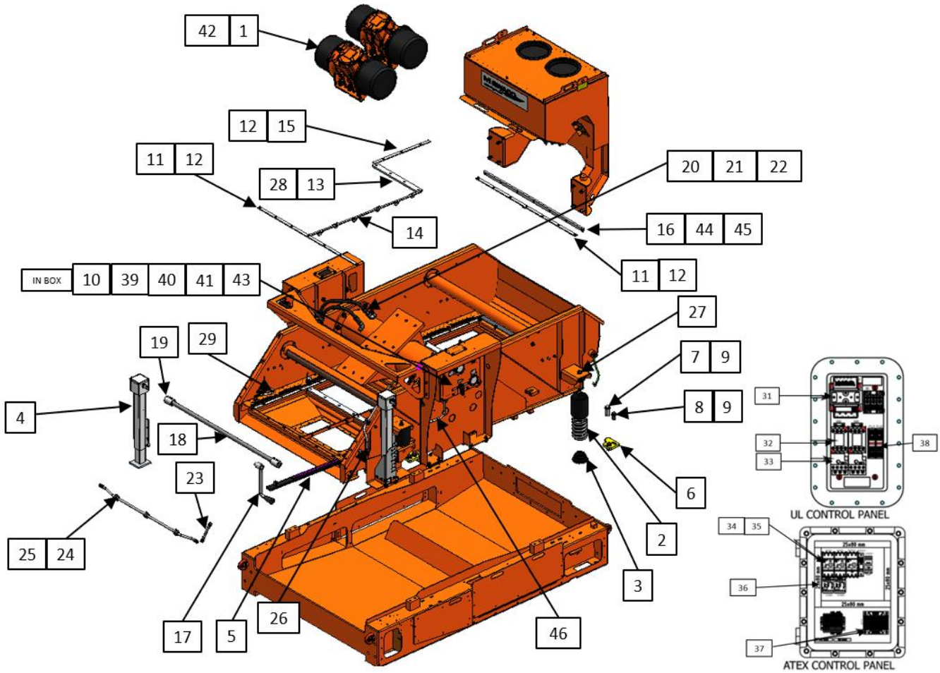
Figure 28. MONGOOSE MAX Shale Shaker Components Exploded View
