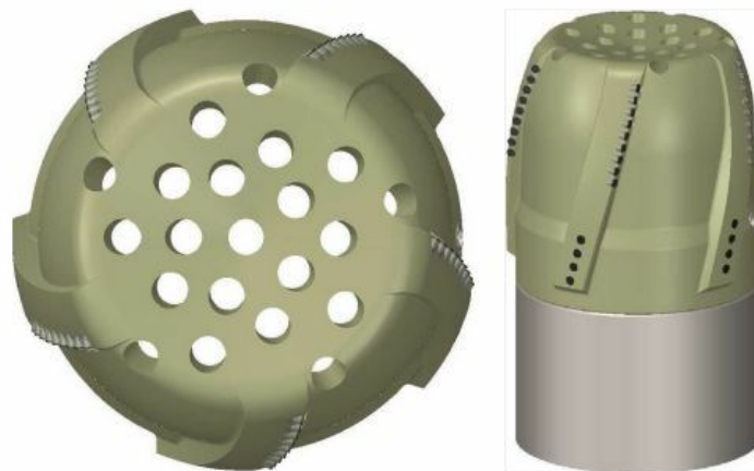
13.375 x 15.5-in XCDR 513 reamer
