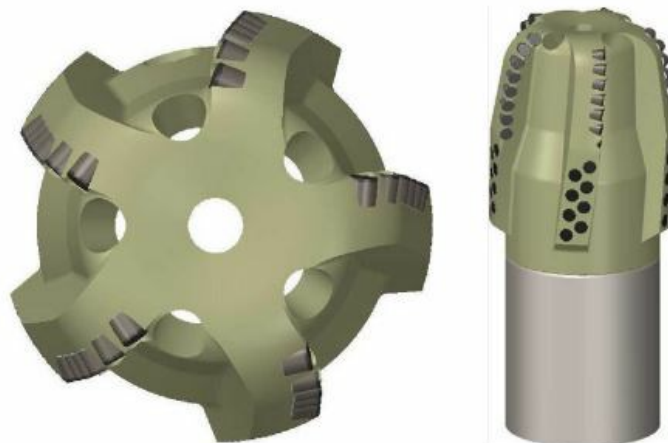
5.5-in x 7.875-in XCD 513 reamer.
