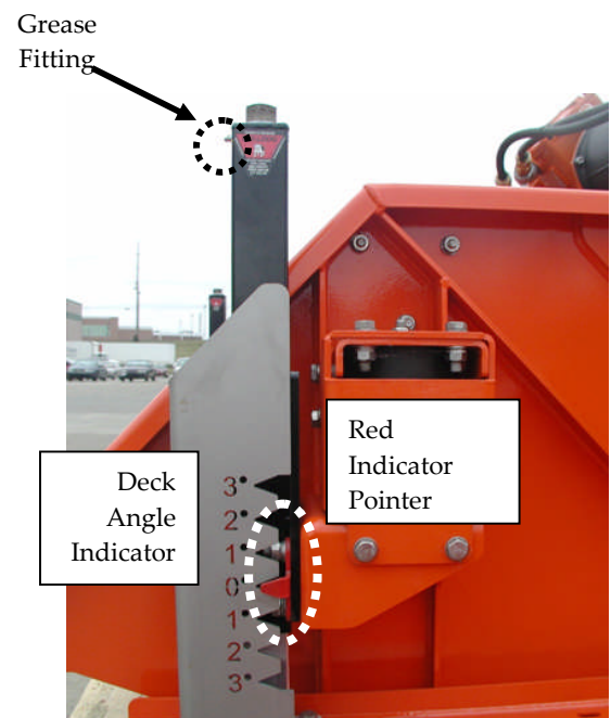
Figure 29 Grease Fitting
