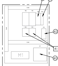
2 MOTOR ATEX STARTER ASSEMBLY LAYOUT
