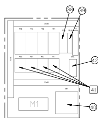
3 MOTOR ATEX STARTER ASSEMBLY LAYOUT
