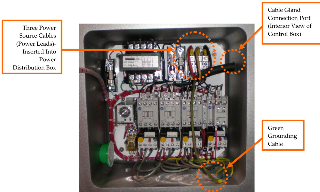
Figure 12 Connection to Outside/External Power (Interior View of Control Box)
